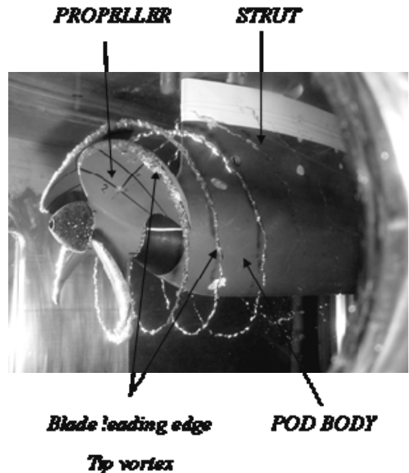
Figure 3. Attached blade leading edge tip vortex cavitation observed on a podded propulsor model set at 0^\circ azimuthing angle
