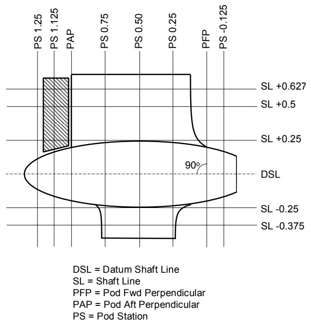
Figure 2. Sample grid definition to describe location and extend of cavitation on pod housing (to be applied on both sides of the housing)
