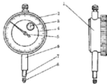
Fig. 1 Dial gauge (with the reading in 0.01mm)
