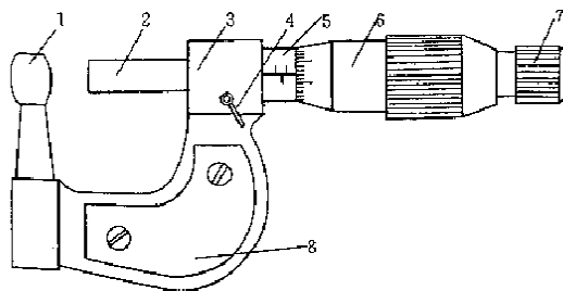
Figure 4 □-type micrometer for wall thickness measuring
