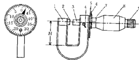
Figure 6 Micrometer for plate thickness measuring with dial
