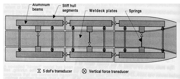
Fig. 2 – Set-up of a hydroelastic catamaran model.
