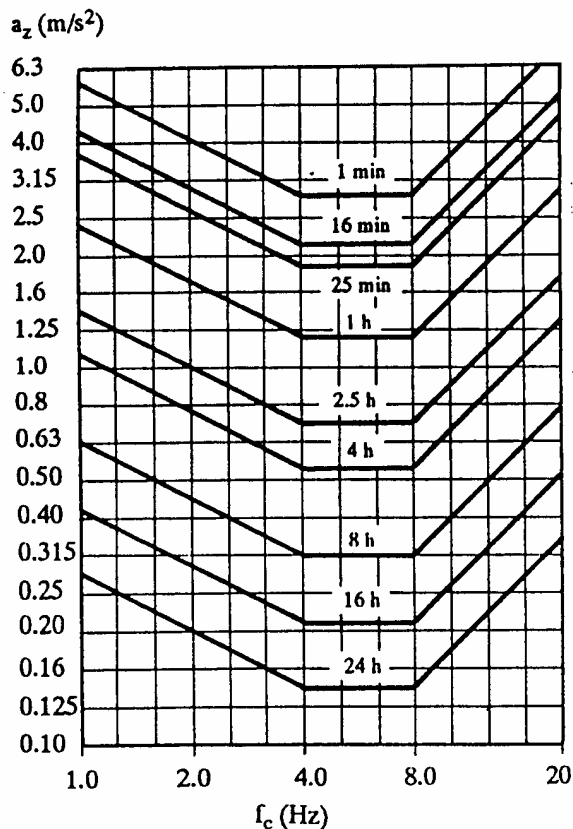
Figure 2. ISO 2631/1 Fatigue-Reduced Proficiency Boundaries
