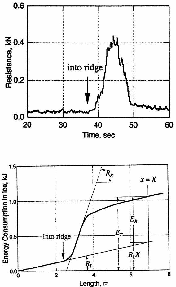
Fig. 2-2. The measured ridge resistance and the definition of ridge resistance based on the energy integral (Izumiyama & Uto 1995)
