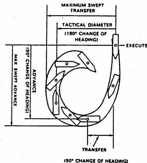
Fig.2-1 The definition of quantities used in turning circle tests
