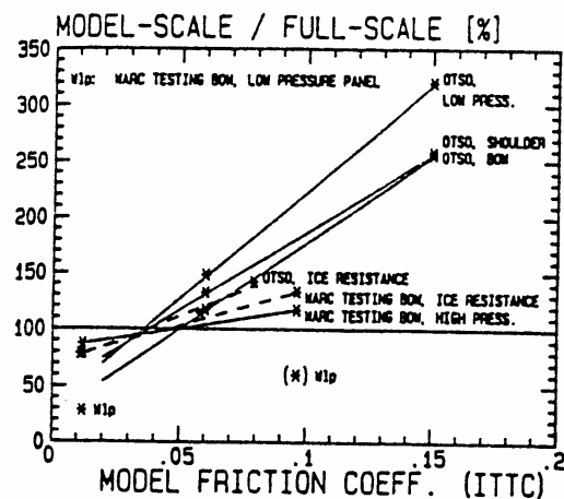
Fig. 4 The ratio between extrapolated model scale ice resistance and measured full scale ice resistance plotted versus the coefficient of friction in model scale (Liukkonen 1989).
