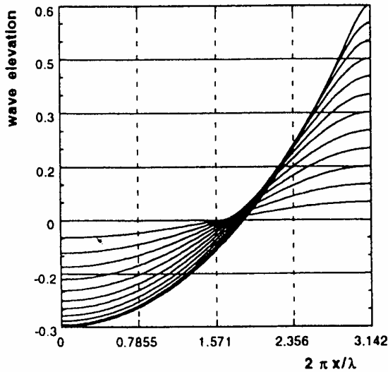
Figure1 Variation of Wave Profile with Wave Amplitude (Shallow Water Waves).
